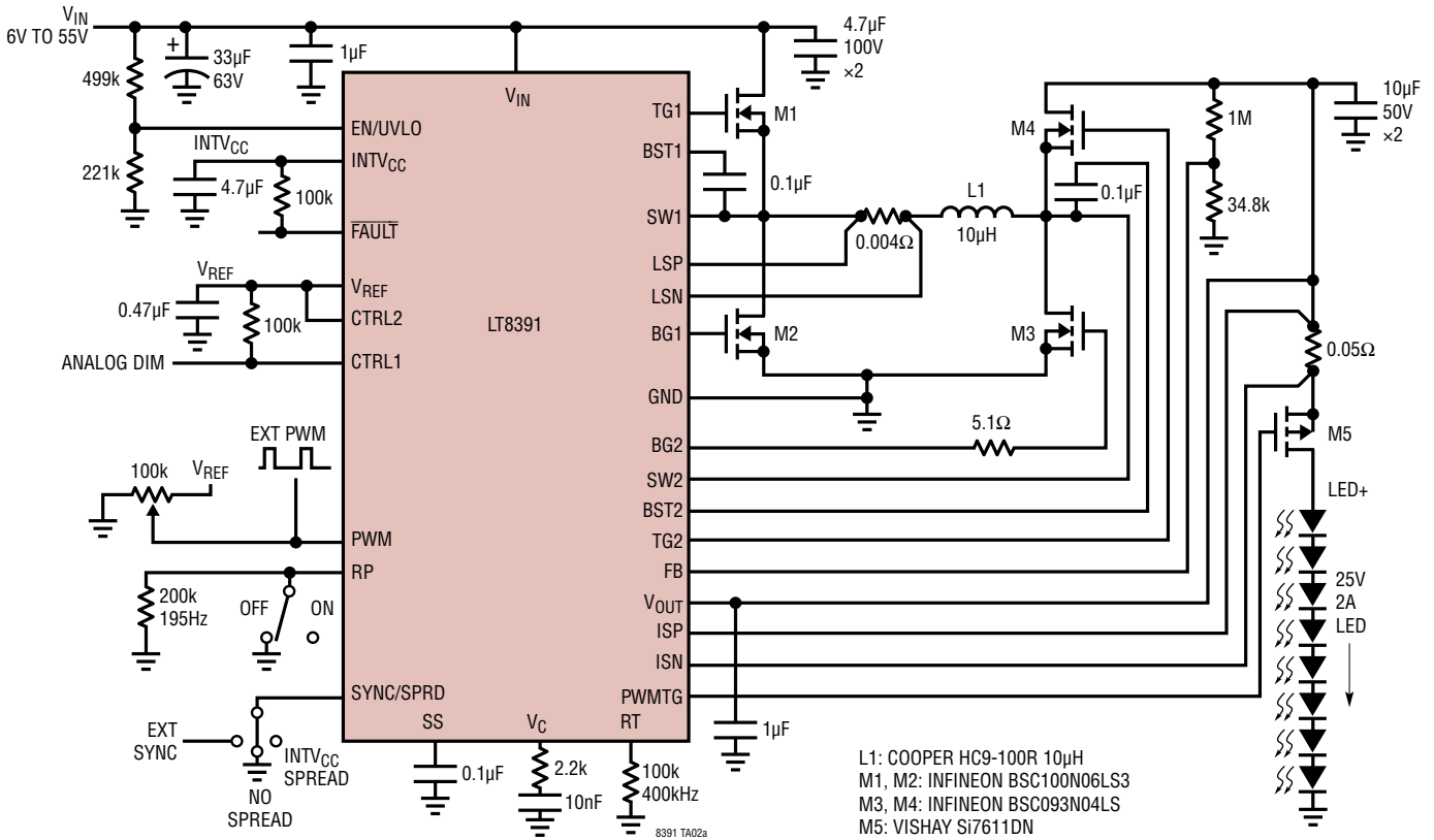
100Hz 1000:1 External PWM Dimming ( V_{IN} = 36V )
