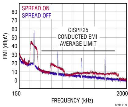
Figure 9. Conducted Average EMI Comparison
